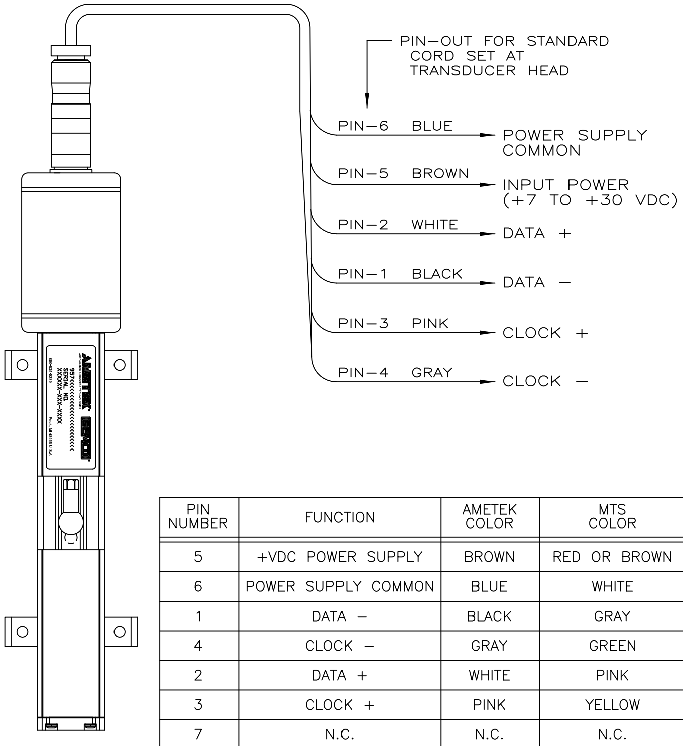
Figure 3-7: Wiring for Connector Option "M", 7 Pin DIN
