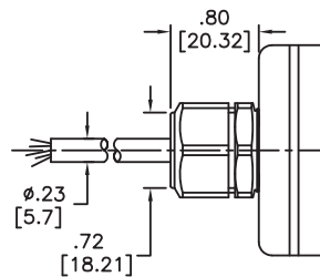
CONNECTOR OPTIONS C &amp; H
