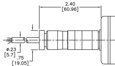
CONNECTOR OPTIONS M &amp; B
