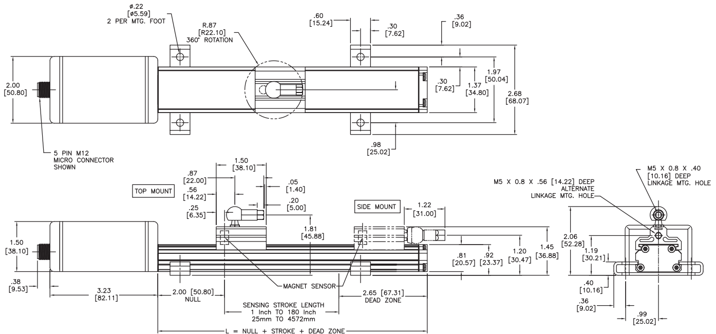
Figure 1-1 957SSI Dimension Drawing for Reference
